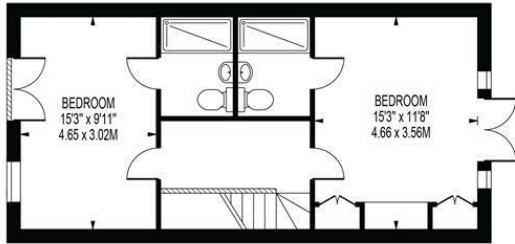
SECOND FLOOR
